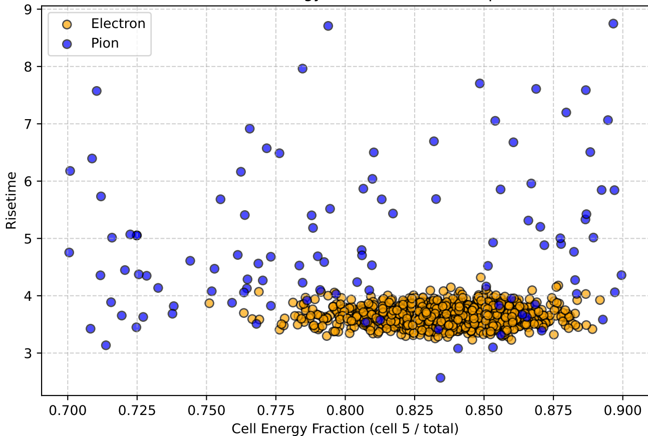
Risetime vs Cell Energy Fraction for 5.0GeV particles
